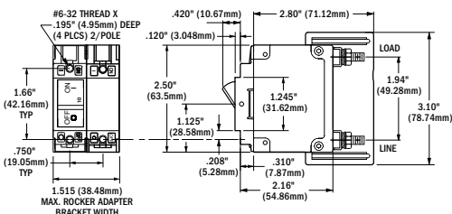
7464 UL-489 Flat Rocker
