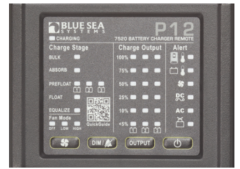
P12 Battery Charger Remote Display
