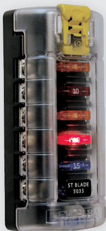
LED ON indicates blown fuse Shown in ST Blade Fuse Block PN 5035
